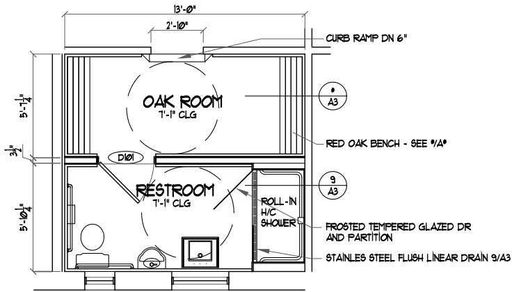
2 FIRST FLOOR RESTROOM A3 SCALE: 1/4" = 1'-0"
