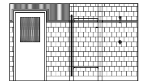
8 RESTROOM ELEVATION SCALE: 1/4" = 1'-0"
