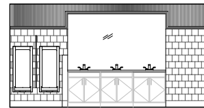
3 RESTROOM ELEVATION SCALE: 1/4" = 1'-0"
