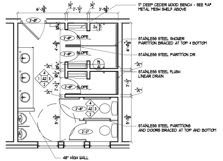
2 THIRD FLOOR R.R. PLAN SCALE: 1/4" = 1'-0"
