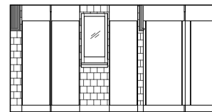
4 RESTROOM ELEVATION SCALE: 1/4" = 1'-0"
