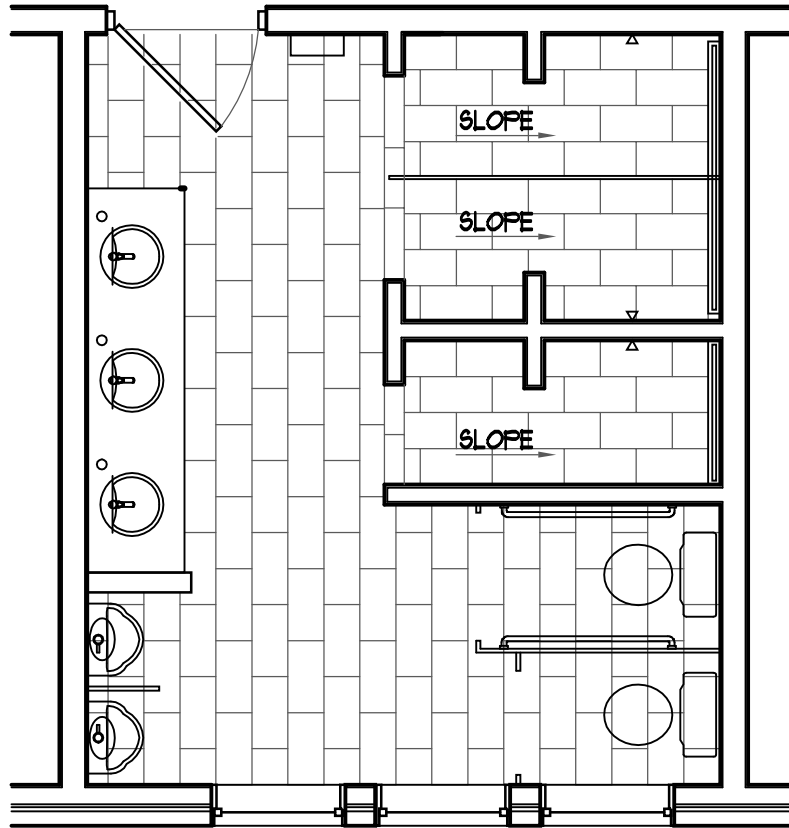
2 THIRD FLOOR R.R. PLAN SCALE: 1/4" = 1'-0"
