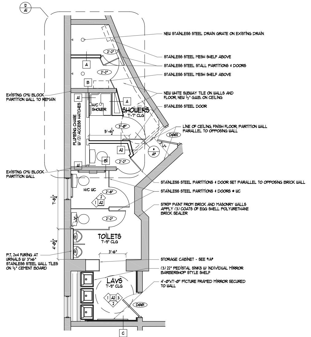
4 BASEMENT BATH FLOOR PLAN A1 SCALE: 1/4" = 1'-0"
