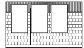
7 RESTROOM ELEVATION SCALE: 1/4" = 1'-0"
